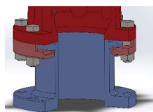
Breakaway Traffic Kit
